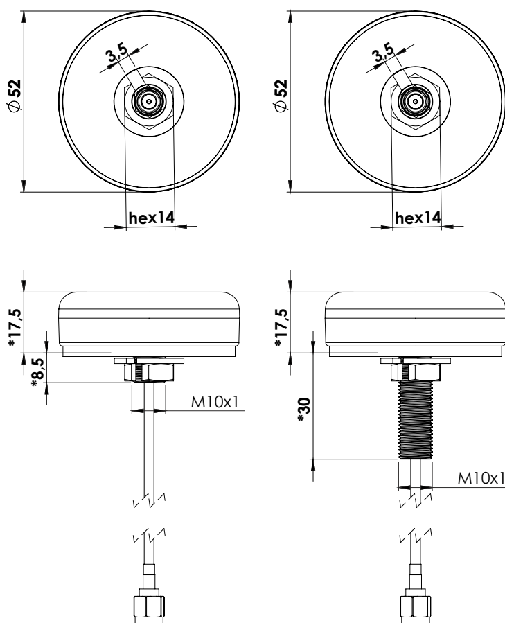
2J4704B-TH8,5 8,5 mm Thread
