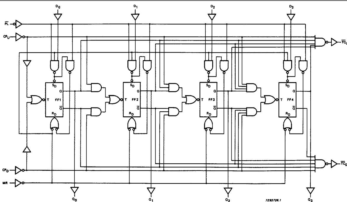
Fig.6 Logic diagram.
