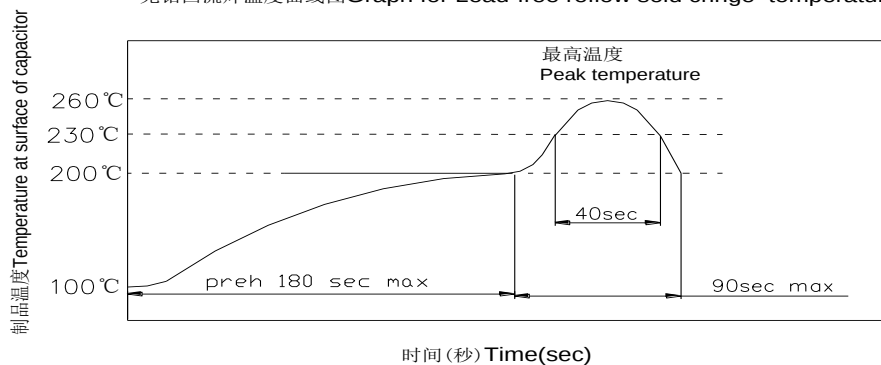
无铅回流焊温度曲线图 Graph for Lead-free reflow sold cringe temperature
