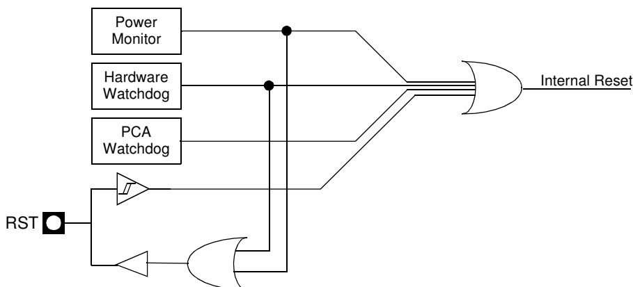
Figure 10-1. Reset schematic
