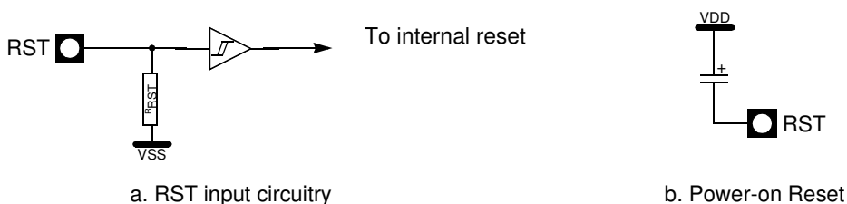
Figure 10-2. Reset Circuitry and Power-On Reset
