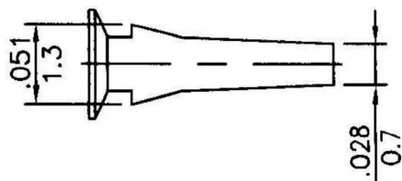
Polarizing Plug
