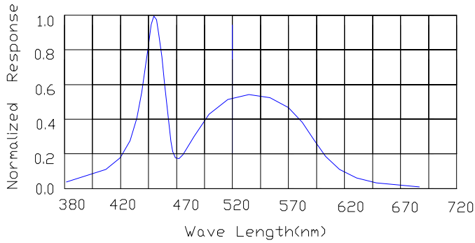
Spectral Reduance
