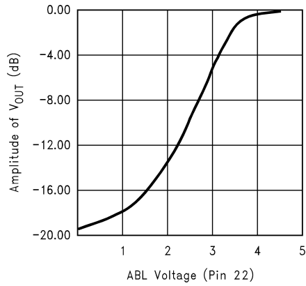
ABL Attenuation
