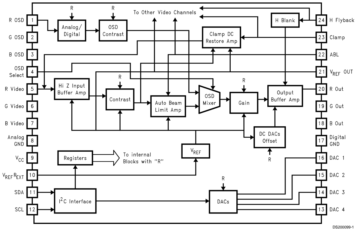
FIGURE 1. Order Number LM1269NA See NS Package Number N24N
