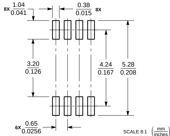
Figure 14. Micro8™
