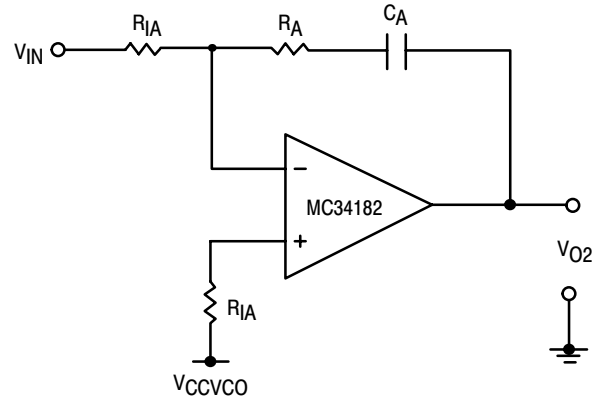
Figure 7. Integrator Subsection
