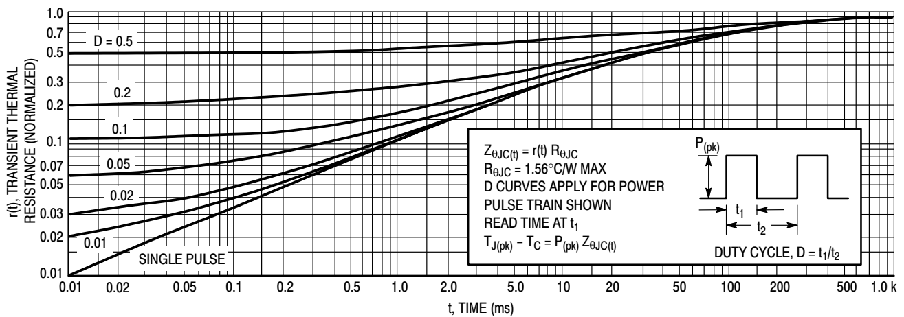
Figure 2. Thermal Response
