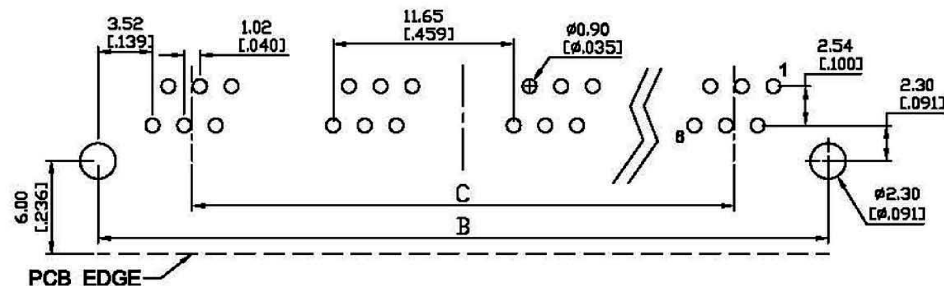
SUGGESTED PCB LAYOUT TOP VIEW
