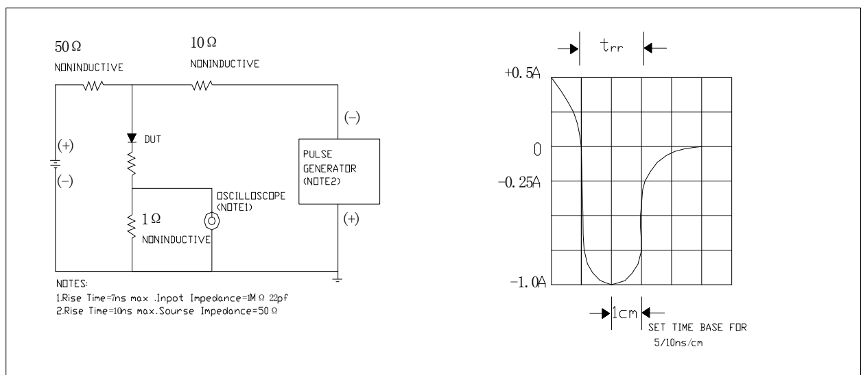
FIG.5 反向恢复时间试验电路及测试波形示意图 Diagram of circuit and Testing wave form of reverse recovery time
