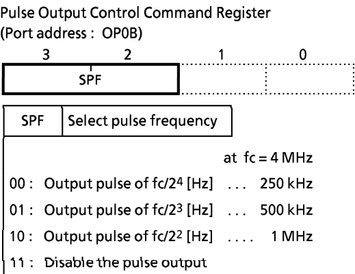
Figure 3-17. Pulse Output Command Register
