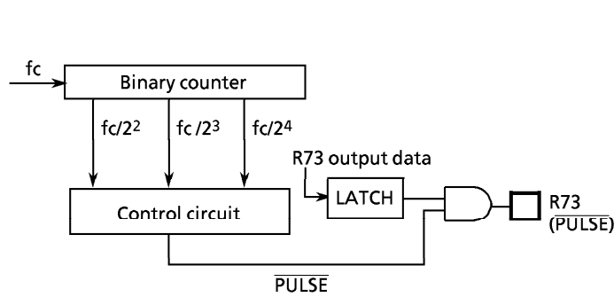
Figure 3-16. Pulse Output Circuit
