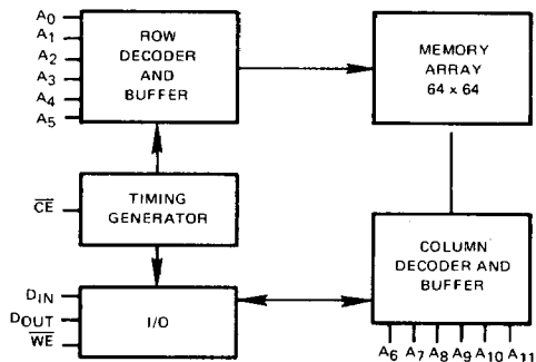
BLOCK DIAGRAM
