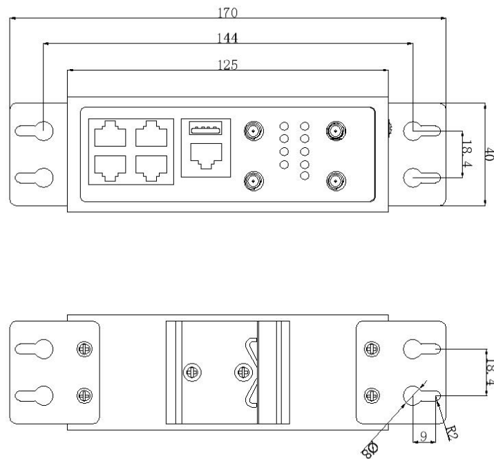
Figure 1 USR-G809 Dimensions
