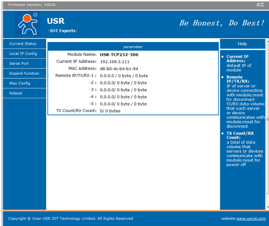
Figure 27 Web Server
