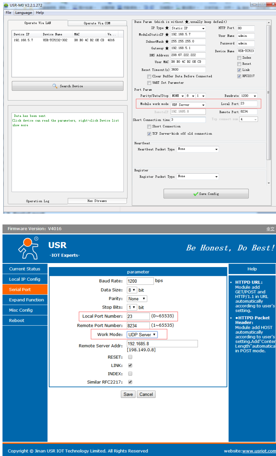
Figure 13 UDP Server
