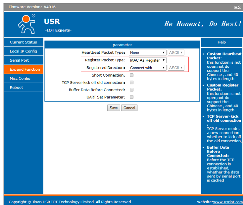
Figure 18 Identity Packet
